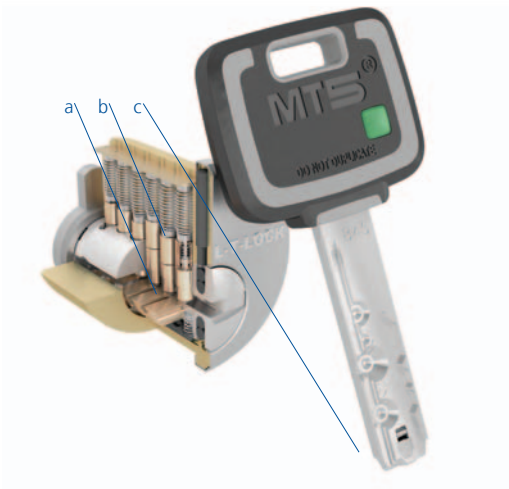
a - Mul-T-Lock telescopic pin technology b - Side bar locking mechanism with unique horizontal finger pins c - Patented mobile interacting Alpha Spring
